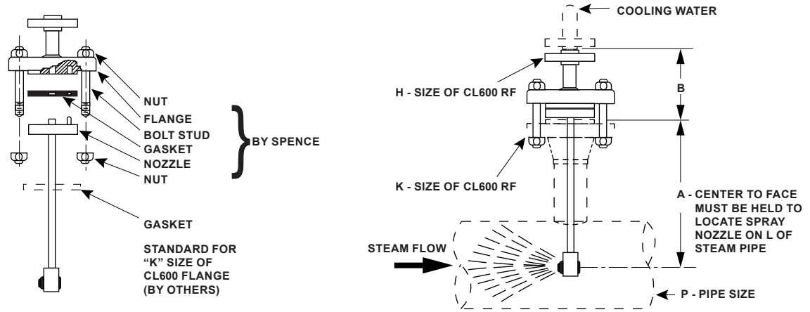
Figure 3. Air-Operated, Mechanical-Atomizing Desuperheater Dimension
