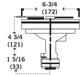
TYPE A54 19 LBS (8.6 KG)
