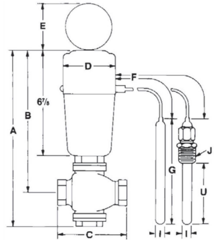
TYPE 2010-2040 DIRECT AND REVERSE ACTING
