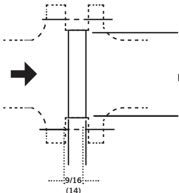
ANSI 250, 300 AND 600 FLANGED
