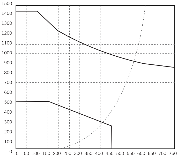
PRESSURE/TEMPERATURE CHART
