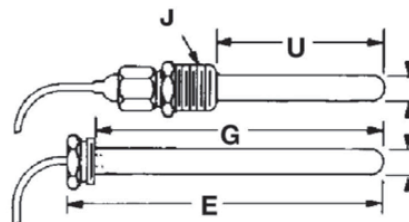
GAS SERVICE BULB AND WELL DIMENSIONS INCHES (MM)
